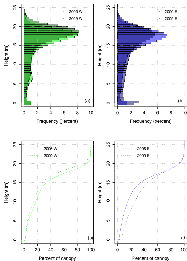
Figure 6. Histograms of canopy top height (m) derived from aerial lidar for the east sector (blue bars) and west (green bars) for (a), (b) 2006 and 2009; cumulative frequency of canopy top height for (c) west sector in 2006 and 2009 and (d) east sector in 2006 and 2009 at the Straits Inclosure, Alice Holt Forest.
